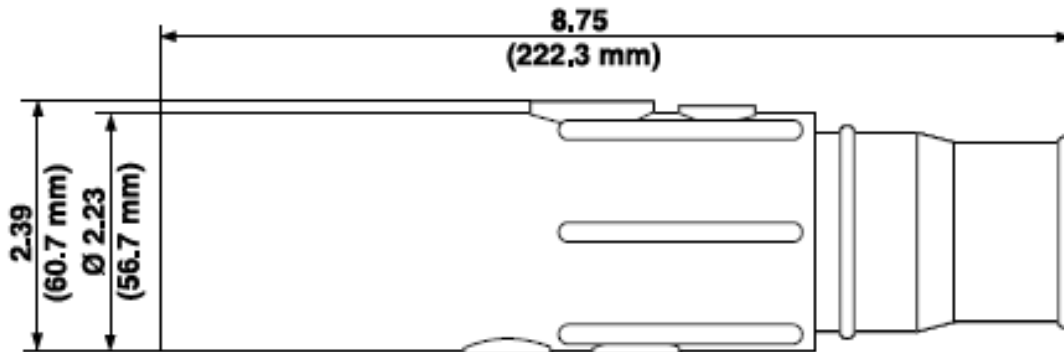
Male Plug - Double Set Screw Detachable
