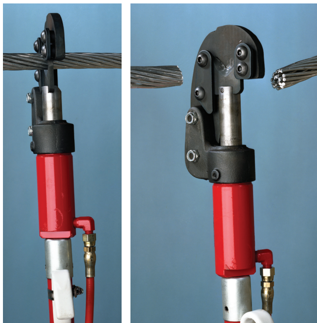
Hook-style jaw hangs on conductor to help position tool. Guillotine-type blades result in smooth, clean cuts.
