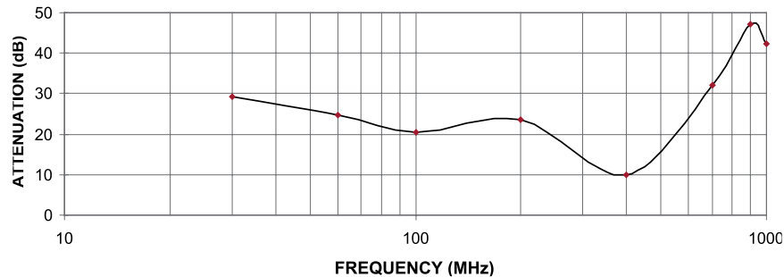
Q1286PEMC QLINE D Enclosure Shielding Effectiveness
